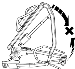
Shallow 4-Point Cradle
